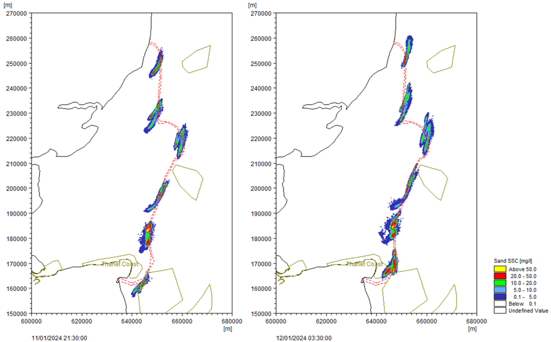
Plate 1.41 Sand SSC levels for jetting installation commencing on spring tides with output on flood (left) and ebb (right) tide after first 24 hours of activity
