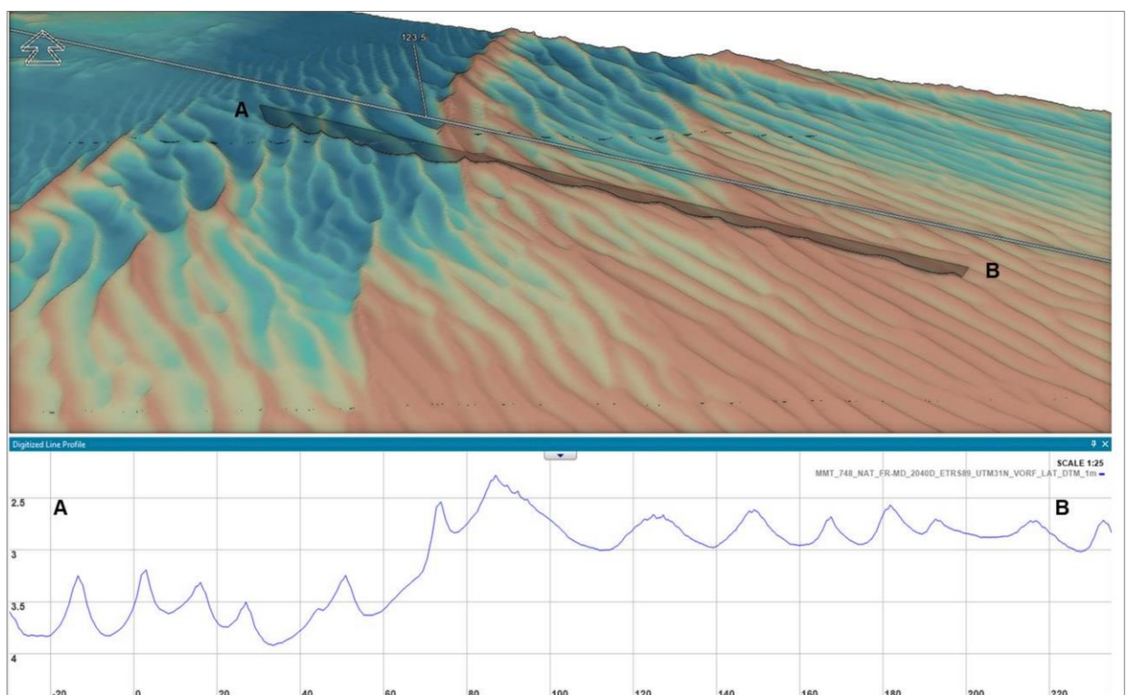
Plate 1.34 Mega ripples up to 3.53 m high located near KP 108 (MMT, 2022)
